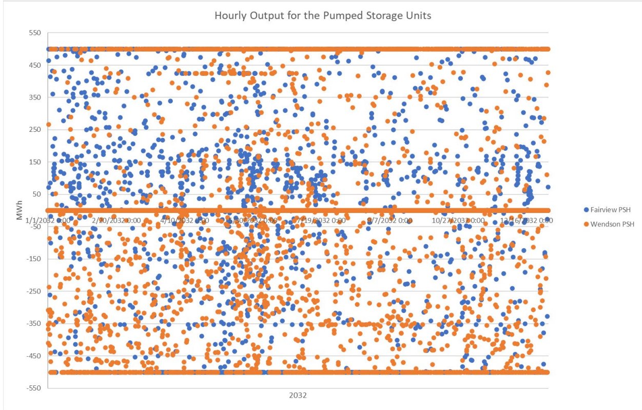
5 6 Figure 3: Raw output for the Rye Development pumped storage units
